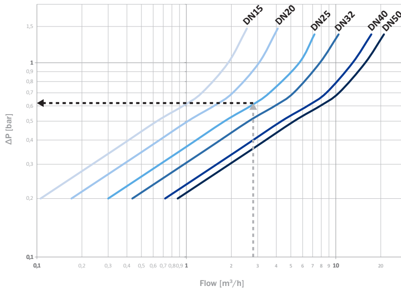
FLOW DIAGRAM - \Delta P
